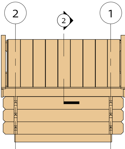
Roof 2
